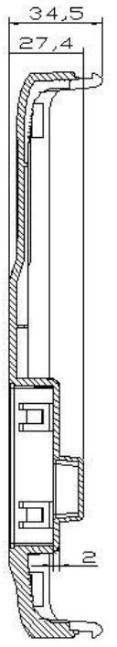
SECTION C-C
